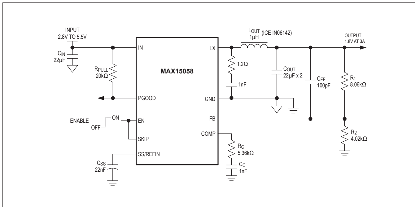
Figure 6. Application Circuit for Skip Mode Operation
